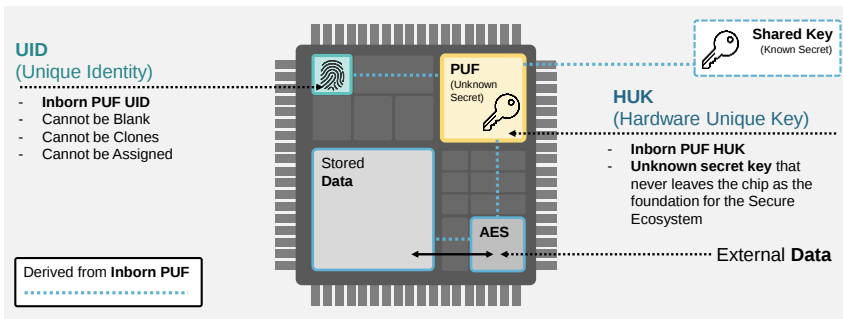
Figure 3-3 PUF-supported functions.
