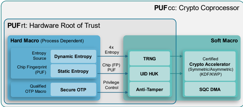
Figure 5-1 PUFcc architecture.
