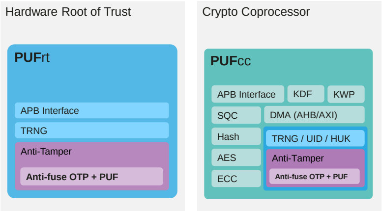
Figure 6-4 Root of trust and crypto coprocessor from PUFsecurity.
