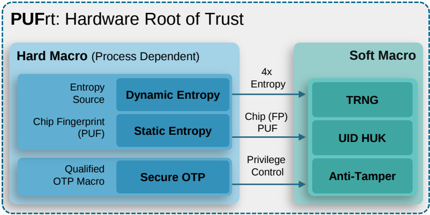
Figure 4-2 PUFrt architecture.
