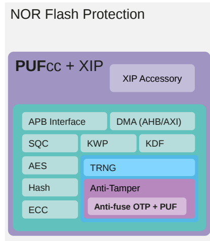
Figure 5-6 PUFcc and XIP accessory module.
